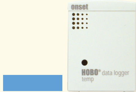
HOBO U10-001 Size/Weight: 6.0 x 4.7 x 1.9 cm (2.4 x 1.9 x 0.8")/28 g (0.9 oz)
