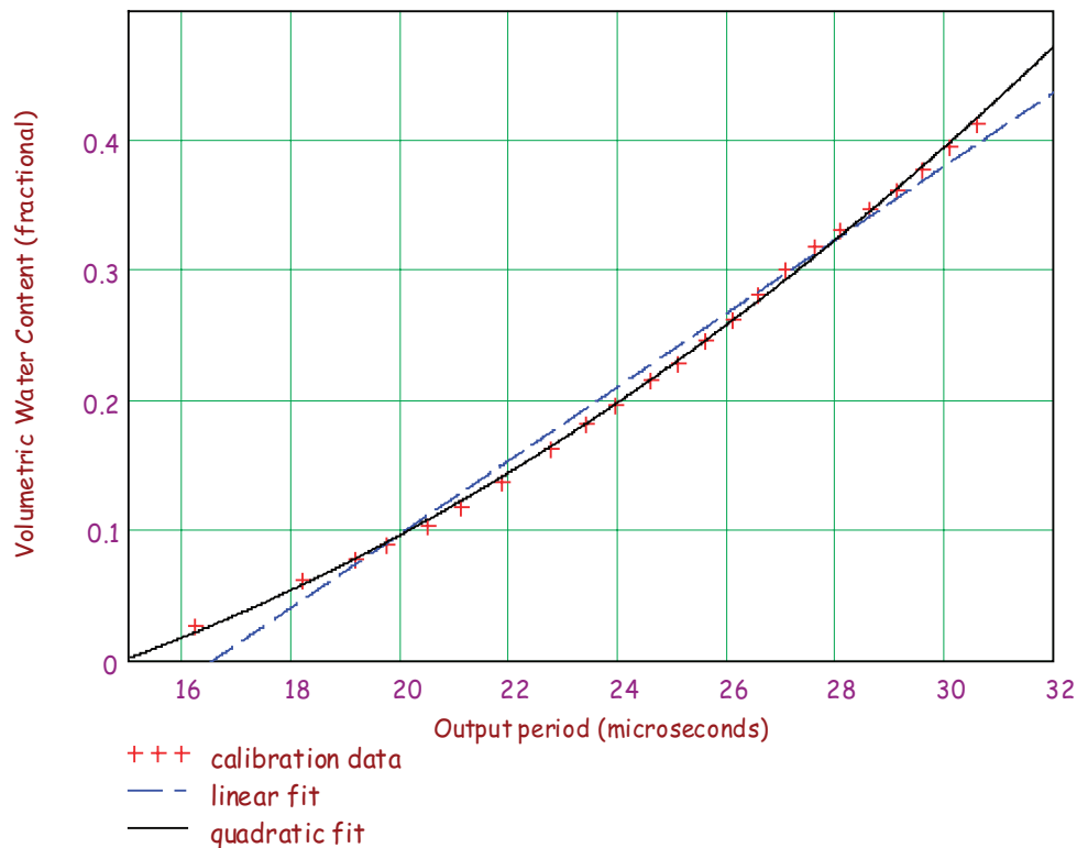
Figure 1. CS625 linear and quadratic calibration derived from loam soil.
