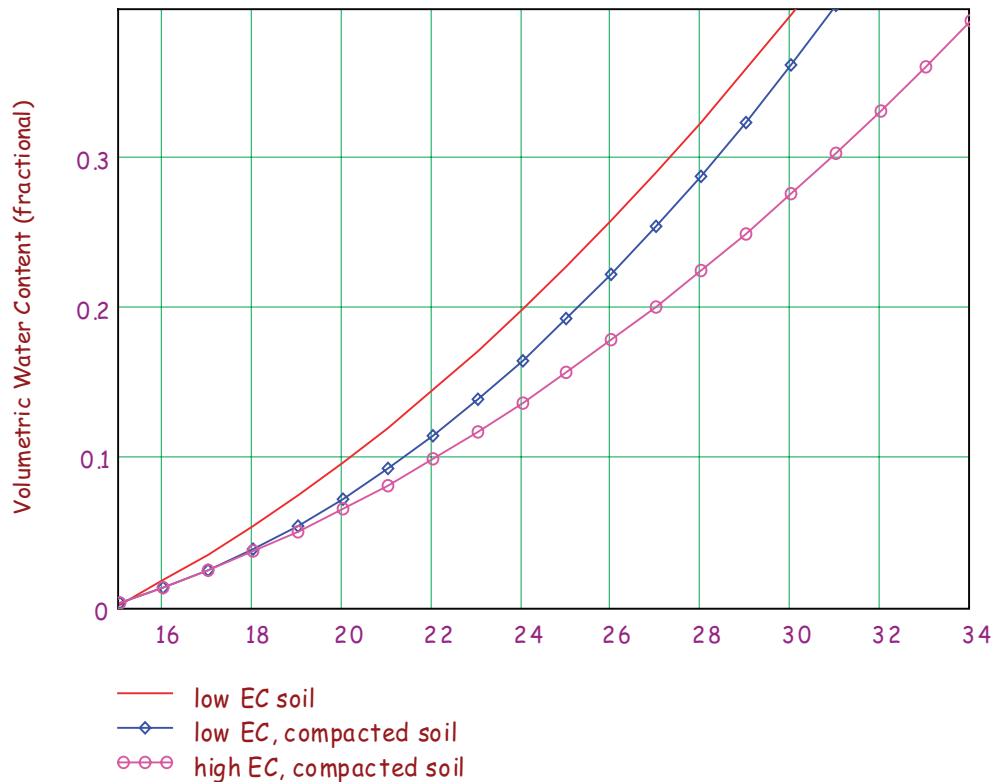
Figure 2. CS625 response in compacted, sandy clay loam soil and low EC loam for comparison.
